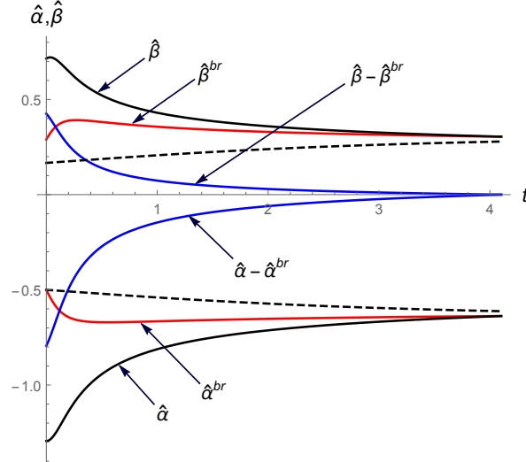
Figure 2: Learning and Signaling Incentives, (r, \sigma, n, \bar{p}, T, g_0) = (0, 1, 2, 1, 4.1, 2) .
