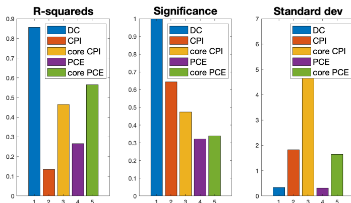
Figure 4: Summary statistics for rolling Phillips curve regressions
