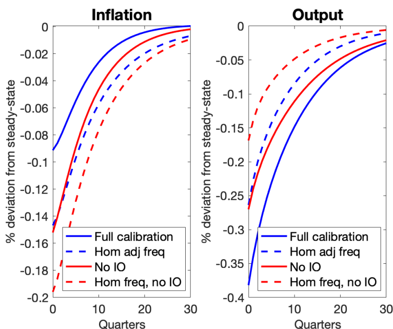
Figure 2: Impulse response to a 10 bp nominal rate shock
