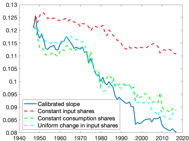
Figure 1: Slope of the Phillips curve over time
