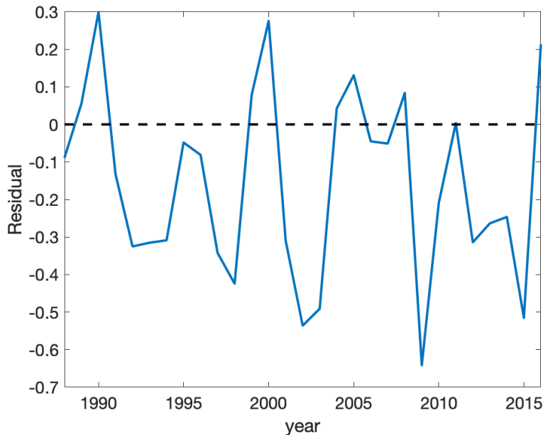
Figure 3: Time series of the endogenous residual
